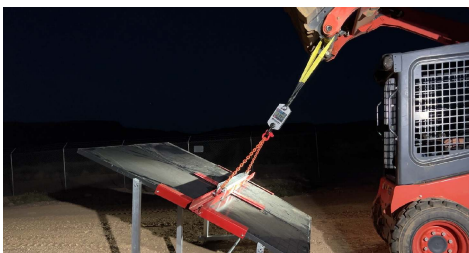
PHOTO 7: IR-30 Solar Racking System at max load
