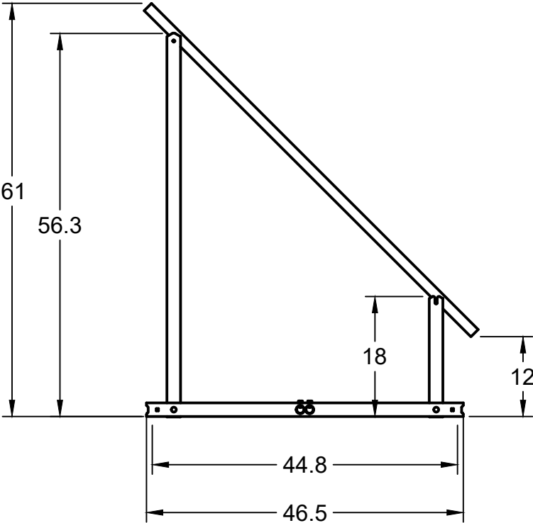
AnchorSpike hole-to-hole dimension: 44.8 inches
